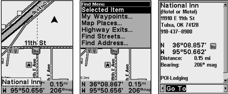
A POI selected by the cursor, left, The Find Menu, center, POI information screen, right.
